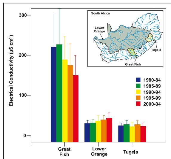
Figure 40. Electrical conductivity at three long term river water quality monitoring stations in South Africa. Bars represent mean ( \pm 1 standard deviation) conductivity over five-year intervals between 1980 and 2004.
