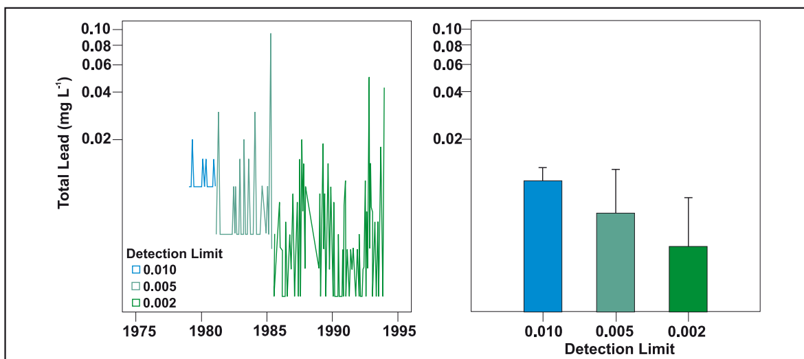
Figure 48. Example of changing analytical detection limits over time and the effects on observed mean concentrations. Data are total lead measurements from the Seine River in Paris, France, between 1979 and 1993 (left panel). Mean lead concentrations ( \pm 1 standard deviation; right panel) of samples collected during each 'detection limit period' suggest decreasing concentrations over time, but it is difficult to conclude if the trends are real or due to improved analytical techniques and detection limits over the same period.
