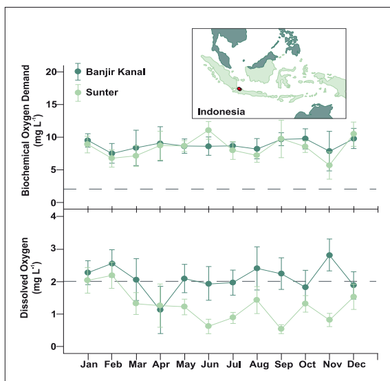
Figure 19. BOD and DO in two Indonesian rivers, plotted as monthly means ( \pm 1 standard error). Dashed lines indicate the BOD concentration below which a system is considered to be unpolluted and the DO concentration below which most fish die (Chapman, 1996). Note that both rivers are typical of polluted systems BOD concentrations are well above the threshold for unpolluted systems, and DO concentrations are near or below the level at which most fish die.
