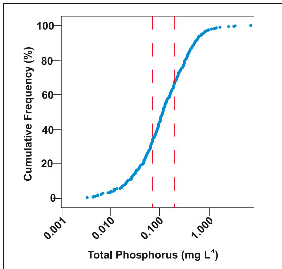
Figure 12. Cumulative frequency diagram of mean total phosphorus concentrations in river monitoring stations. Dashed lines separate distribution of global data into thirds, which can be used to classify systems as oligotrophic (bottom third), mesotrophic (middle third) or eutrophic (upper third). The table shows the boundary concentrations that divide rivers by region.
