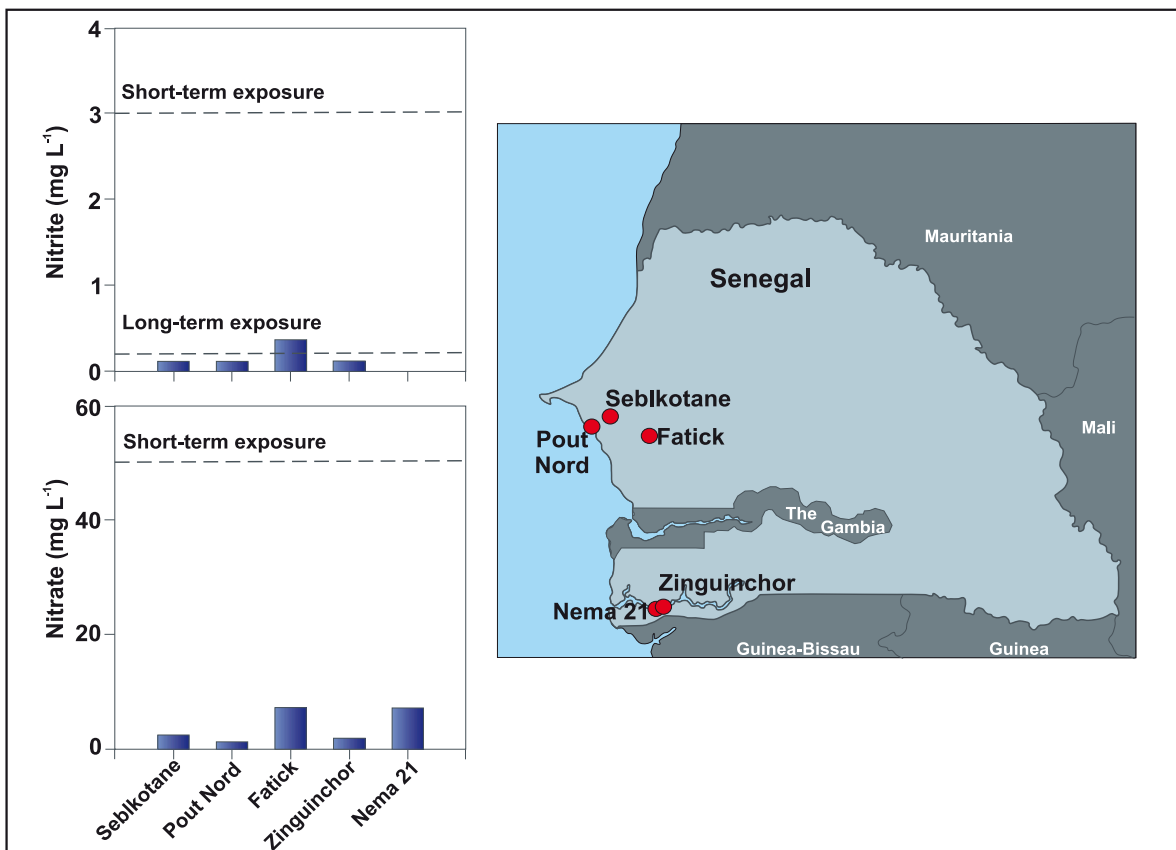
Figure 30. Nitrite (top panel) and nitrate (bottom panel) concentrations in five drilled wells in Senegal. Dashed lines indicate WHO drinking water guidelines to protect against methaemoglobinaemia in infants caused by short term exposure to nitrate and nitrite, and a provisional guideline for long-term exposure to protect against adverse health effects in humans. Note that although none of the samples exceed short term nutrient exposure guidelines, nitrites in the Fatick well, in particular, exceeded the provisional water quality guideline.
