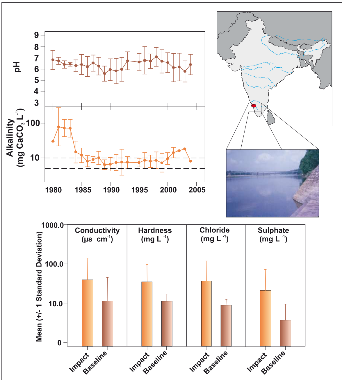
Figure 35. Top panel: Trends in annual mean ( \pm 1 standard deviation) pH and alkalinity in the Periyar River, India, 500 m downstream from a rare earth metals processing plant. Dashed lines indicate alkalinity range that is typical of systems that are highly sensitive to acidification. Bottom panel: Comparison of mean conductivity, hardness, chloride and sulphate concentrations between upstream, baseline station and downstream, impacted station in the Periyar River, India. Note that the dramatic decline in alkalinity in the mid-1980s to 'highly sensitive' status corresponds to periods where variability in mean pH concentrations increased (as shown by larger error bars around each mean). Note also that conductivity, hardness, chloride and sulphate concentrations at the impacted station, downstream of the metals processing plant, were consistently greater than the upstream, baseline station.
