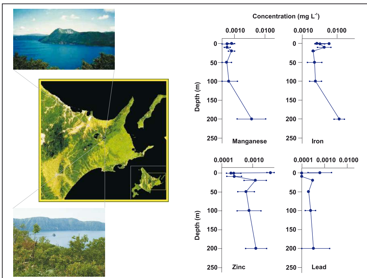
Figure 14. Total metal concentrations plotted against depth in Lake Mashu, Japan, between 1995 and 2002. Data are mean \pm 1 standard deviation. Note the increase in iron and manganese near the lake bottom, where oxidation-reduction states are usually high.
