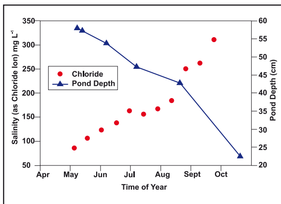
Figure 10. Relationship between salinity (measured as chloride concentration) and pond depth over the course of a growing season in a small, saline pond (Pond 50, St. Denis National Wildlife Refuge) in Saskatchewan, Canada. Data collected in 2000, M.J. Waiser, Environment Canada.
