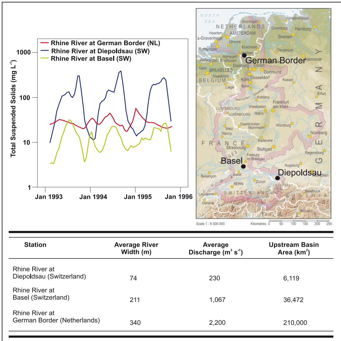
Figure 28. Total suspended solids in the Rhine River near its headwaters in Switzerland at the base of the Swiss Alps (Diepoldsau), on the German-Swiss border near Basel and downstream of Lake Constance, and at the German-Dutch border at the start of the Rhine River delta in the Netherlands. The table shows the characteristics of the river at each sampling point. Note that suspended sediment concentrations are highest and most variable at the most upstream station, where discharge patterns are likely to be erratic and dominated by snowmelt in the Alps. In contrast, suspended sediment concentrations are greatly reduced immediately downstream of Lake Constance, but variability in concentrations remains high. Suspended sediment concentrations are slightly higher at the most downstream point of the river, but much less variable, probably due to the regulatory effect of the 21 impoundments located upstream of this station, as well as numerous weirs and other flow control structures along the length of the river.
