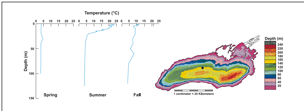
Figure 2. Seasonal patterns in depth profiles of temperature in Lake Ontario, Canada, with data from 1993. Note the approximately uniform and cool temperatures in spring (May), the strong thermocline between approximately 10 and 25 m depth during the summer months (June - September), and the breakdown of the thermocline in the fall months to cooler and more uniform temperatures (October).
