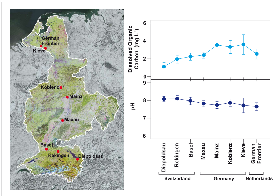
Figure 18. Dissolved organic carbon (DOC) and pH along the length of the Rhine River and flowing through Switzerland, Germany and the Netherlands. Note the general increase in DOC and the concurrent slight decrease in pH along the length of the river.
