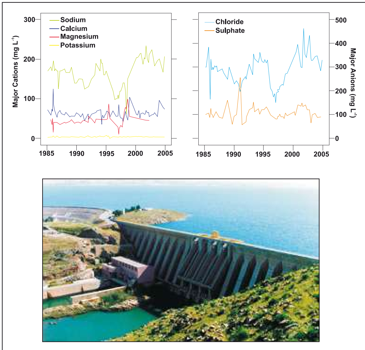
Figure 11. Concentrations of major cations (left panel) and anions (right panel) in the surface waters of Al. Massira Reservoir, Morocco, between 1985 and 2005. Carbonate and bicarbonate concentrations were not measured over the sampling period. Note the similarity in temporal patterns of sodium and chloride concentrations.
