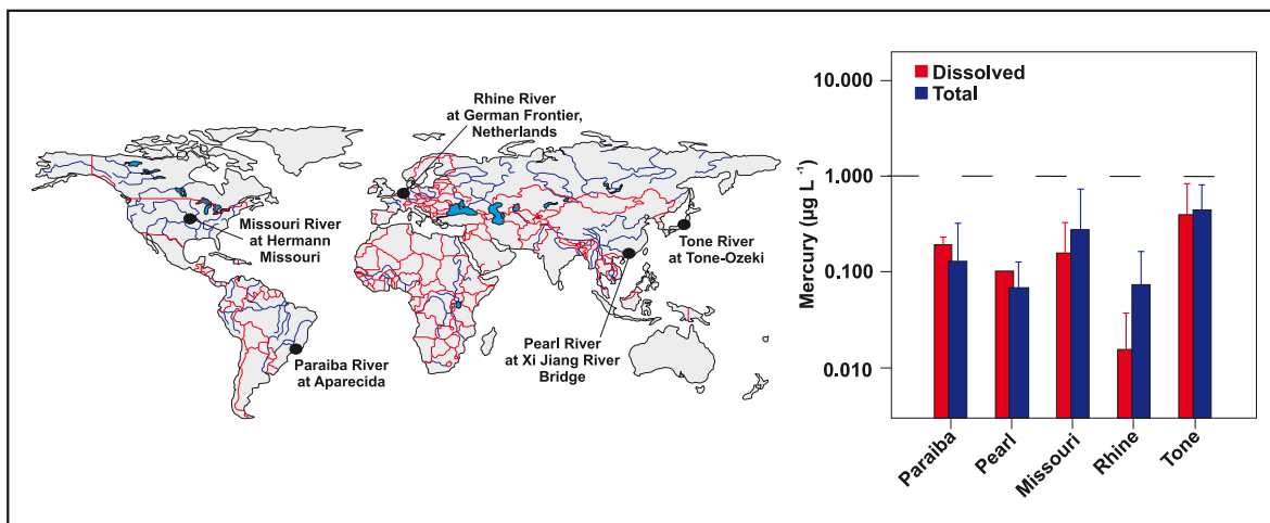
Figure 16. Dissolved and total mercury concentrations in rivers of Brazil (Paraiba), China (Pearl), United States (Missouri), Netherlands (Rhine) and Japan (Tone). Data are mean \pm 1 standard deviation. Dashed line is World Health Organization drinking water quality guideline for total mercury. Note that mean mercury concentrations are below guideline values at all monitoring stations.
