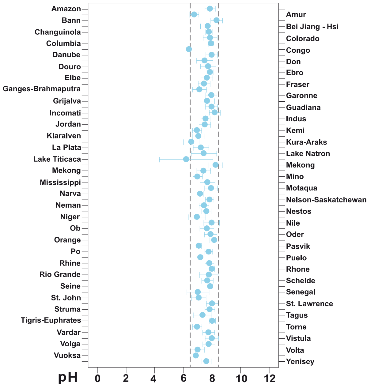
Figure 6 graph. Mean pH ( \pm 1 standard deviation) of major drainage basins in the world. Dashed lines indicate approximate pH range suitable for the protection of aquatic life.
