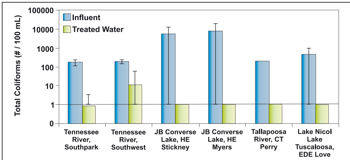
Figure 39. Total coliform concentrations in untreated, influent water and treated water at six water treatment facilities in Alabama, USA. Data are averages ( \pm 1 standard deviation) of monthly samples collected between July 1997 and December 1998. The solid black line is the limit of analytical detection.
