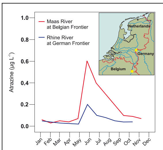
Figure 24. Atrazine concentrations in two rivers of the Netherlands, sampled in 1994. Atrazine is an herbicide used to control weed growth. It is commonly detected in surface and groundwaters. Note the peak in concentrations at both stations around June, when atrazine was most likely applied to the surrounding landscape for weed control. Concentrations at both stations were consistently below the World Health Organization drinking water quality guideline for atrazine of 2 µg L -1 . Because of human health concerns surrounding the detection of atrazine in drinking water supplies, its use has been banned in several countries, including the Netherlands.
