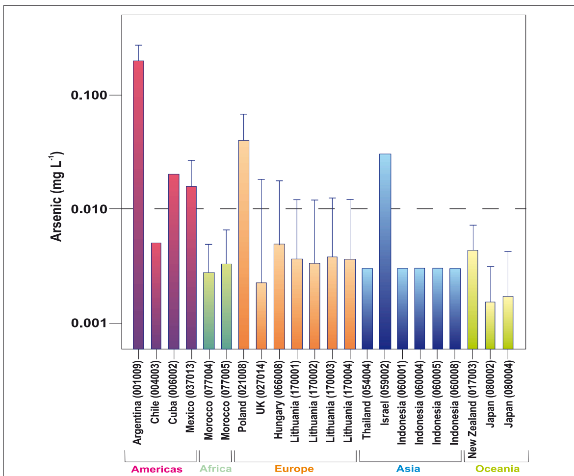
Figure 15. Arsenic in groundwater samples from monitoring stations around the world. Data are mean \pm 1 standard deviation. Dashed line is WHO drinking water quality guideline.
