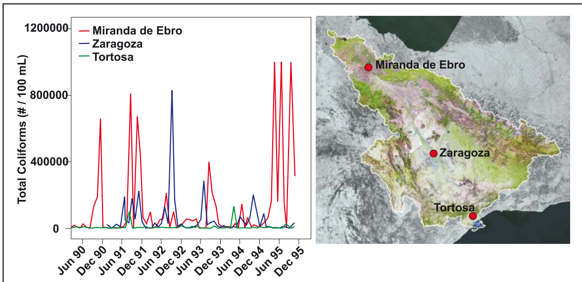
Figure 37. Total coliform concentrations at three monitoring stations in the Ebro River, Spain, measured during the early 1990s.
