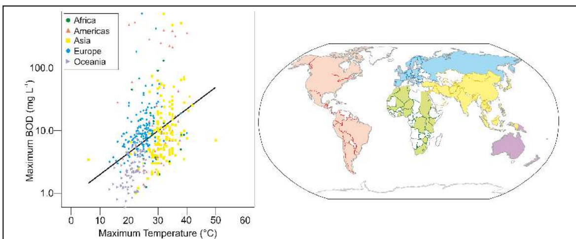
Figure 34. Relationship between maximum reported BOD and maximum reported water temperature at river monitoring stations around the world. The solid line is the 'best fit' relationship between BOD and temperature that can explain approximately 15% of the global variability in maximum BOD. Note that the high degree of uncertainty in the relationship is likely due to variability in concentrations of organic matter that may be found naturally or is released into the water from municipal and rural effluents.
