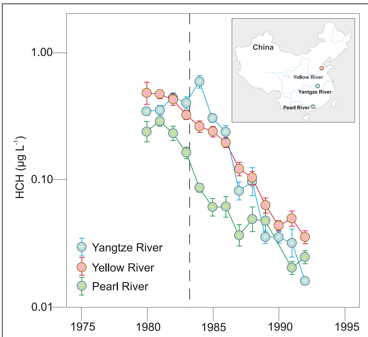
Figure 42. Mean ( \pm 1 standard error) annual concentrations of technical hexachlorocyclohexane (HCH; also known as 'benzene hexachloride' or BHC) in three Chinese rivers between 1980 and 1993. HCH is an organochlorine insecticide that was banned from use in China in its technical form in 1983 (dashed line). HCH is composed of several isomers; the insecticide lindane is composed almost entirely of \gamma -HCH, and was made available in China in 1991 under restricted use (Li et al. , 2001). Lindane is still in use in many parts of the world, and residues have been detected in surface waters.
