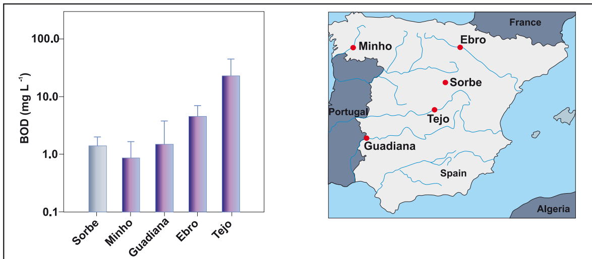
Figure 20. BOD (in mg L -1 ) at one baseline (Sorbe River) and four impact (Minho, Guadiana, Ebro and Tejo Rivers) monitoring stations in Spain. Data are mean \pm 1 standard deviation.
