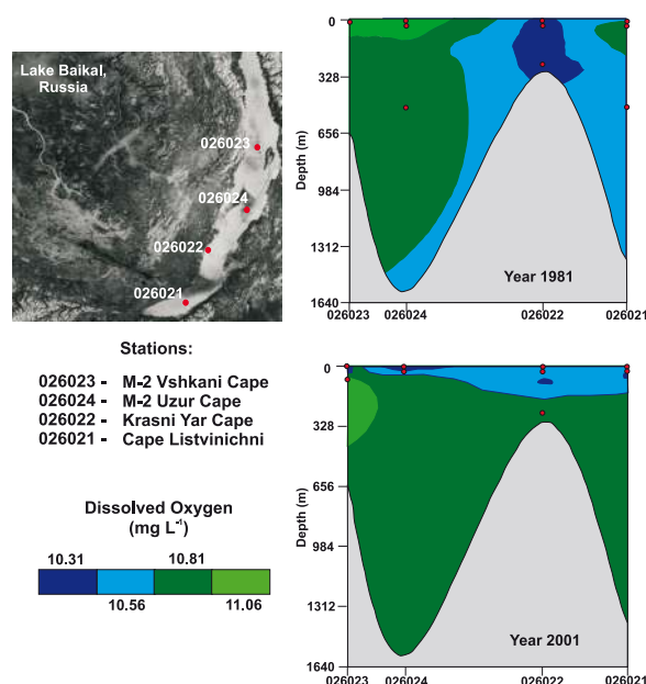
Figure 4. Localized oxygen depression in Lake Baikal, Russian Federation. Note that oxygen depression was more pronounced in Lake Baikal in the shallow basin around Krasni Yar Cape in the early 1980s compared to the early 2000s.
