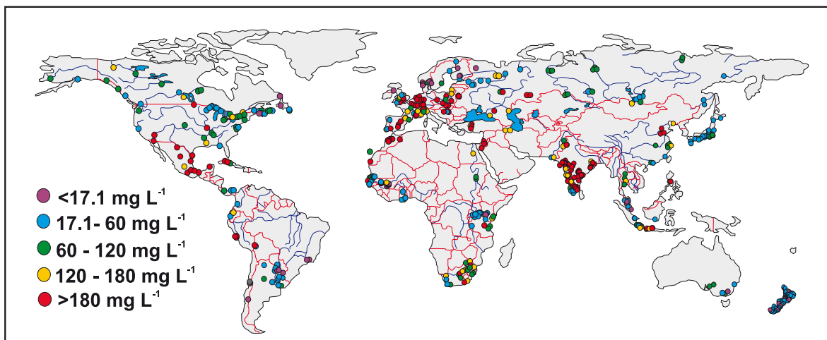
Figure 1. Water hardness ( \text{mg L}^{-1} ) at surface water monitoring stations.
