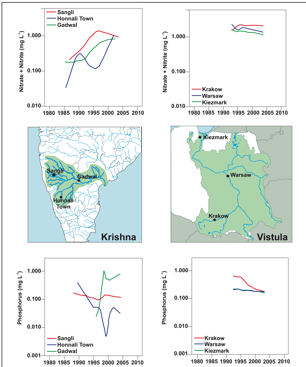
Figure 31. Nitrogen (top) and phosphorus (bottom) trends at river monitoring stations in the Krishna watershed, India, and the Vistula watershed, Poland. Lines represent locally weighted best fit lines to long-term monitoring data.
