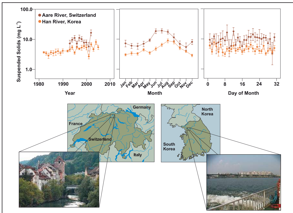
Figure 26. Temporal trends in suspended solids in the Aare River, Switzerland, and the Han River, Korea. Data are annual, monthly, and day of month means with standard deviations.
