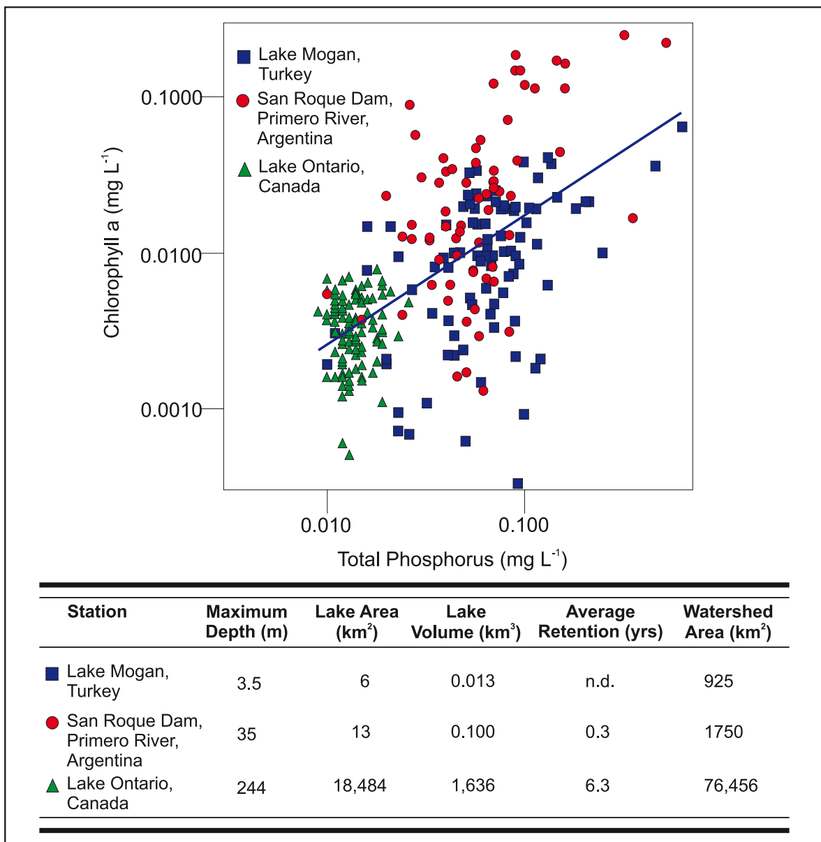
Figure 29. Relationship between biomass of phytoplankton, measured as chlorophyll a, and total phosphorus at three lake and reservoir monitoring stations. Note that despite variability, chlorophyll a increases with phosphorus concentrations and that the relationship is consistent across three systems that vary greatly in physical characteristics. Approximately 40% of the variability in chlorophyll a is explained by this relationship. The solid line is the line of best fit.
