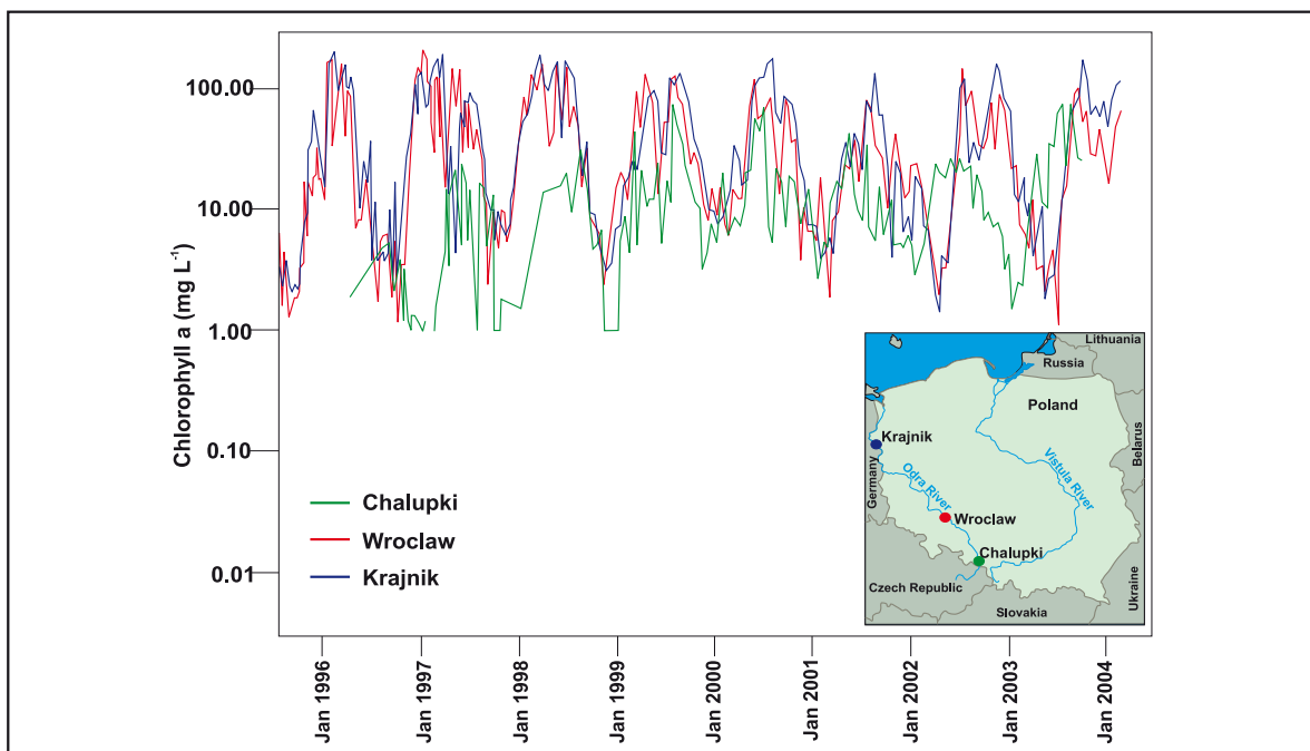
Figure 23. Long-term monitoring of algal biomass, measured as chlorophyll a, at three stations in the Odra River, Poland. Note the strong seasonal cycles in chlorophyll a from year to year at each station.
