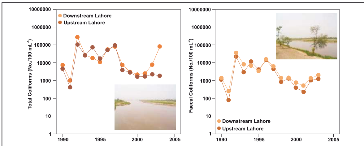
Figure 22. Total and faecal coliform concentrations in the Ravi River, upstream and downstream of the City of Lahore, Pakistan. Data are annual mean concentrations. Note that despite differences being small, coliform concentrations downstream of Lahore are consistently greater than upstream concentrations.
