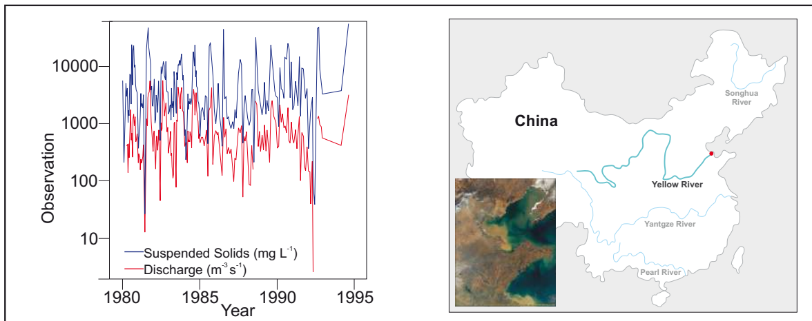
Figure 8. Suspended solids and instantaneous discharge measured in the Yellow River, China, at Lijin, approximately 80 km from the mouth of the river. Note how closely suspended solids concentrations track instantaneous discharge over time.
