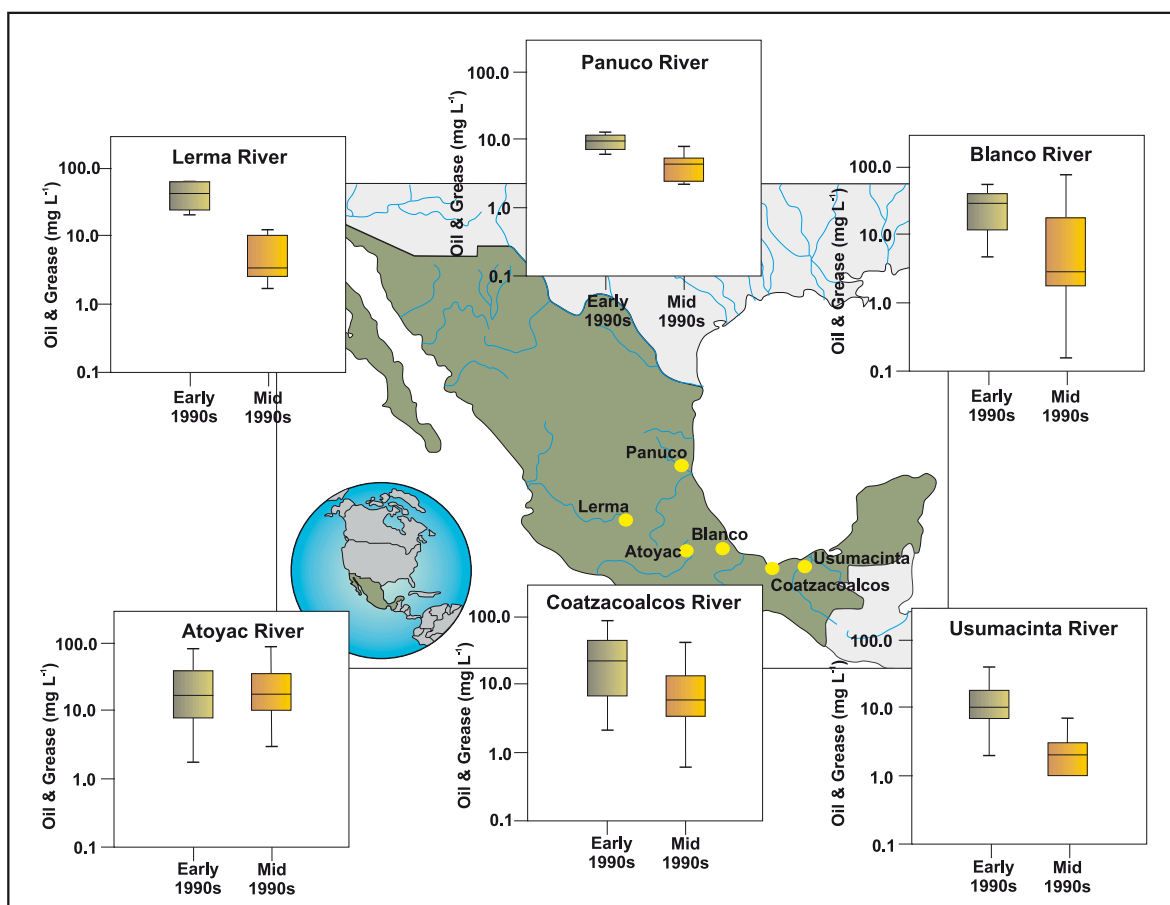
Figure 25. Oil and grease at six river monitoring stations in Mexico. Data collected in early and mid-1990s show a general decline in oil and grease concentrations in most systems over the sampling period. Boxes depict median and 25th and 75th percentiles (mid, bottom, and top of boxes, respectively) and 'whiskers' represent 10th and 90th percentile of data distribution.
