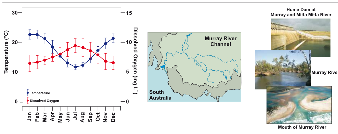
Figure 3. Seasonal patterns in dissolved oxygen and temperature in the Murray River, Australia. Data are monthly means \pm 1 standard deviation. Note that peaks in water temperature coincide with dissolved oxygen minima over the course of a year.
