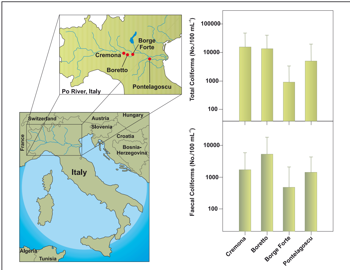
Figure 21. Mean ( \pm 1 standard deviation) total and faecal coliform concentrations at four stations in the Po River, Italy. Data were collected as part of routine monitoring of these stations between 1979 and 1995.
