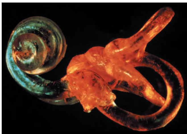
FIGURE 25.7 • Photograph of a cast of the bony labyrinth of the internal ear. The cochlear portion of the bony labyrinth appears blue-green; the vestibule and semicircular canals appear orange-red. (Courtesy of Dr. Merle Lawrence.)
